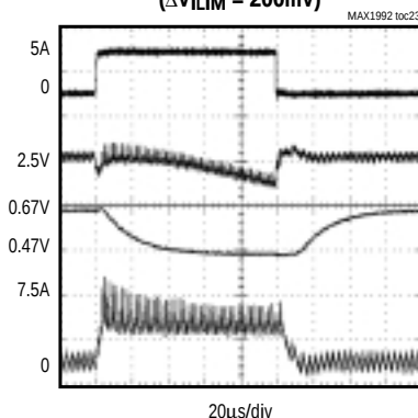
INDUCTOR SATURATION PROTECTION ( \Delta V_{ILIM} = 200mV )
