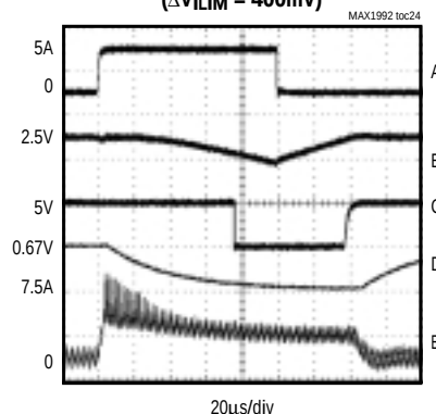
INDUCTOR SATURATION PROTECTION ( \Delta V_{ILIM} = 400mV )
